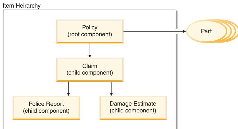
Figure 5. Components hierarchy
