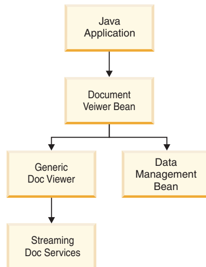
Figure 29. Java application
