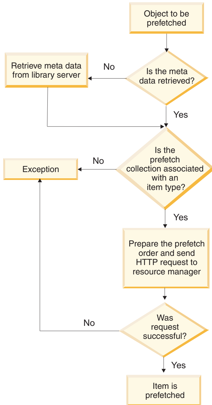
Figure 10. Prefetching objects
