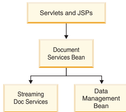
Figure 30. Thin client
