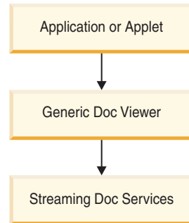
Figure 28. Standalone viewer
