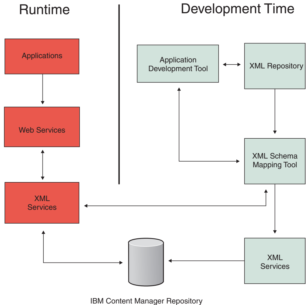
Figure 24. XML services communication flowchart
