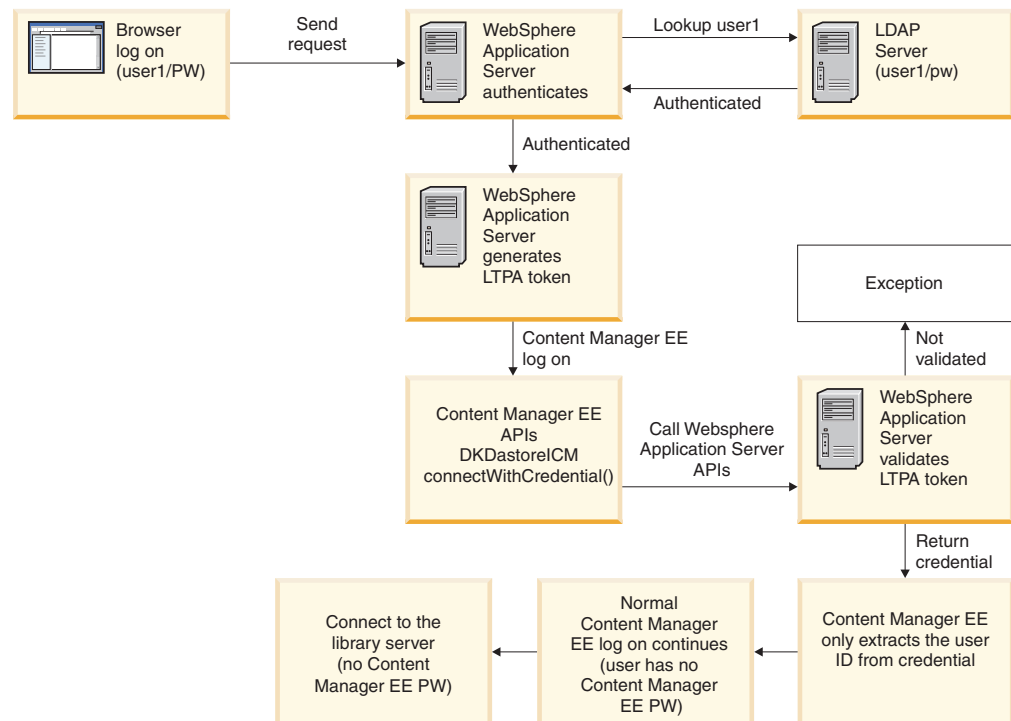
Figure 7. Single sign-on authentication flow in a WebSphere Application Server environment
