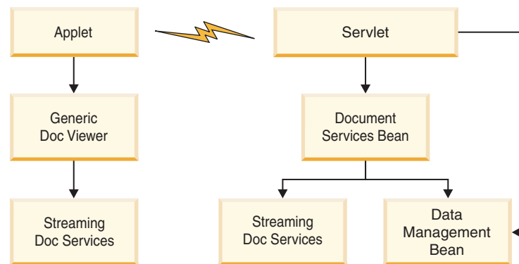
Figure 32. Dual-mode viewer
