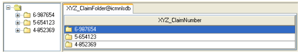
Figure 18. CMBFolderViewer bean
